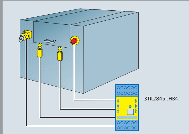
Example 3TK2845-.HB4. Processing station with protective hood and EMERGENCY STOP
