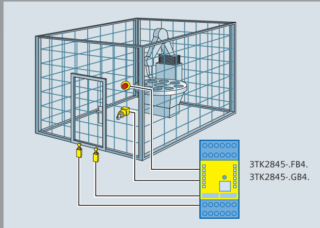
Example 3TK2845-.FB4. /GB4. Robot cell with protective door with tumbler mechanism and EMERGENCY STOP
