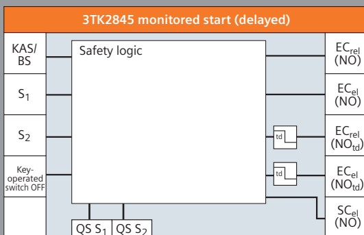
Example 3TK2845-.DB4. Robot cell with protective door and EMERGENCY STOP
