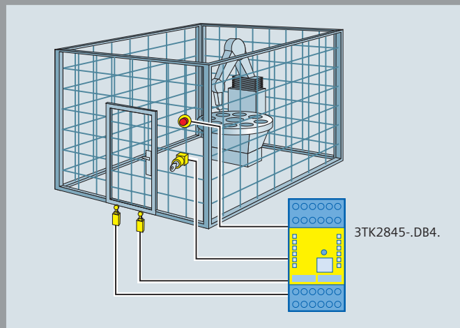
Example 3TK2845-.DB4. Robot cell with protective door and EMERGENCY STOP
