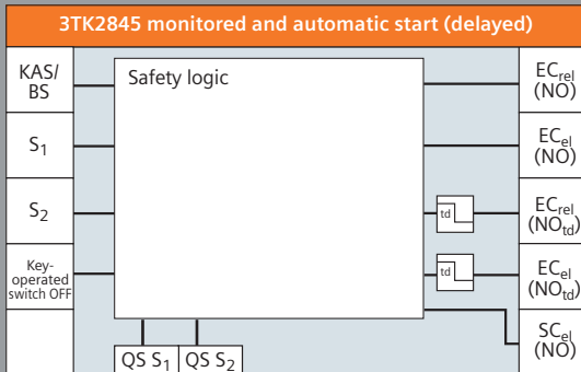
Example 3TK2845-.HB4. Processing station with protective hood and EMERGENCY STOP
