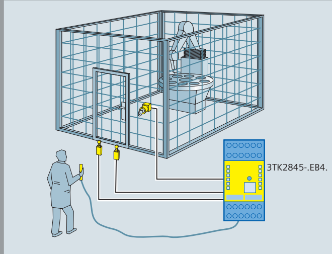
Example 3TK2845-.EB4. Robot cell with protective door and agreement button
